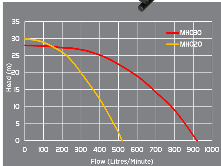
3" POLY PUMP
