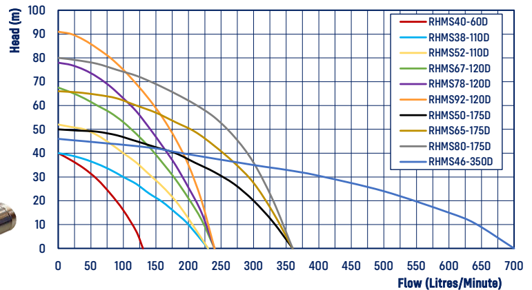
Note: Curves show flow rate with both pump running together
